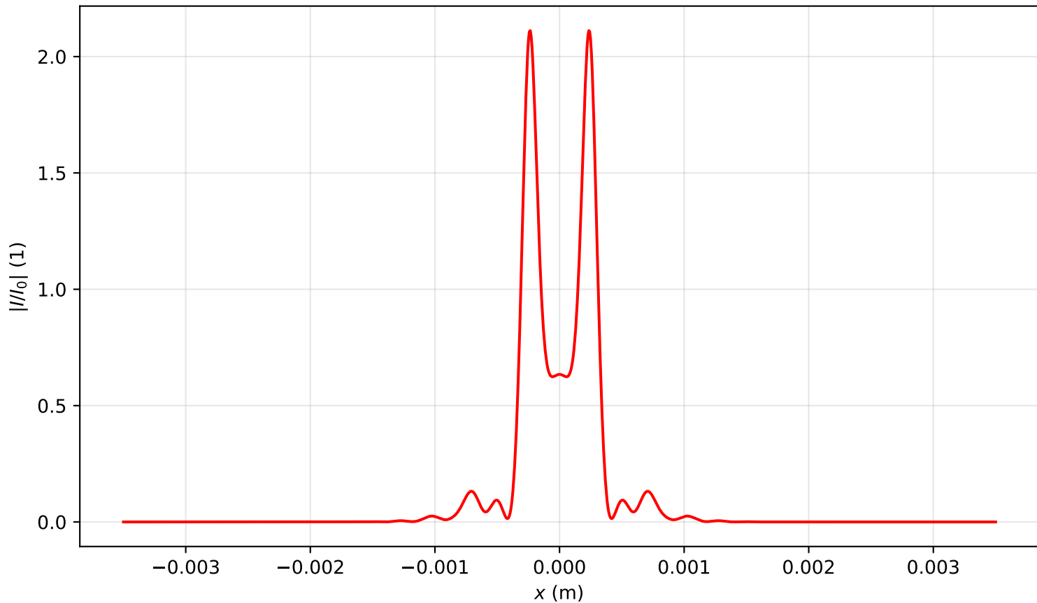
Intensity profile I(x, y = 0, z = 0.716)/I_0 , P_{in}=6.5P_{cr} , artificial time
